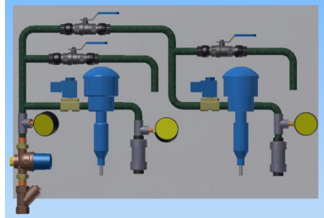
Water Driven Proportional Dosing
